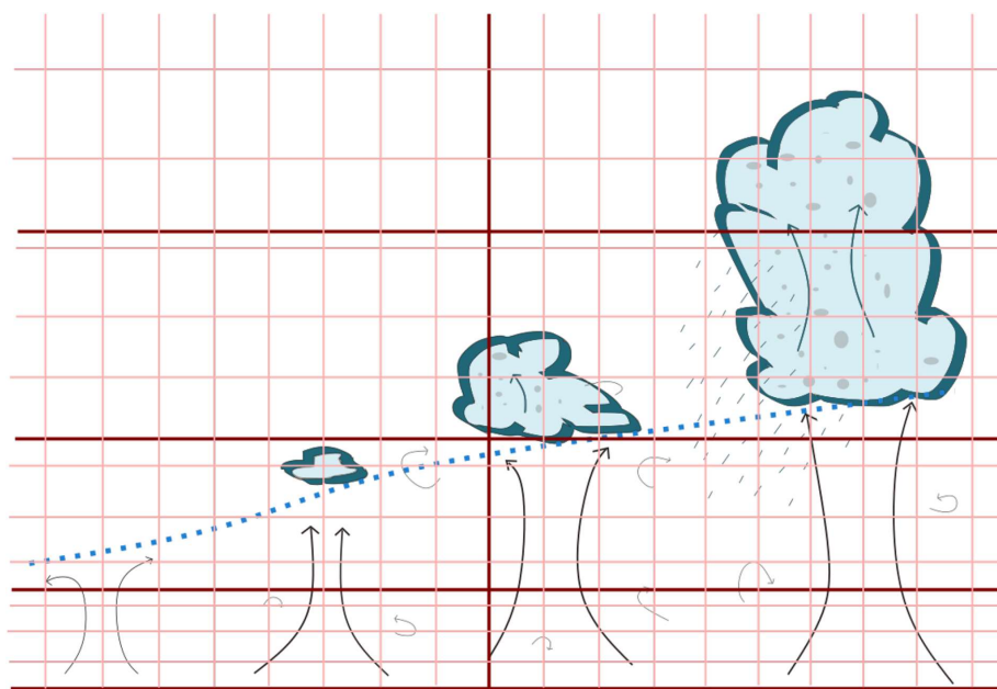
FIGURE 2 Schematic illustration of how a model represents various boundary-layer depths and different cloud sizes between km-scale grid lengths (dark red) and hectometric grid lengths (light red). As the boundary layer deepens, hectometric models are able to represent larger eddies. Similarly they are able to represent growing convective clouds once they become large enough. [Colour figure can be viewed at wileyonlinelibrary.com ]
