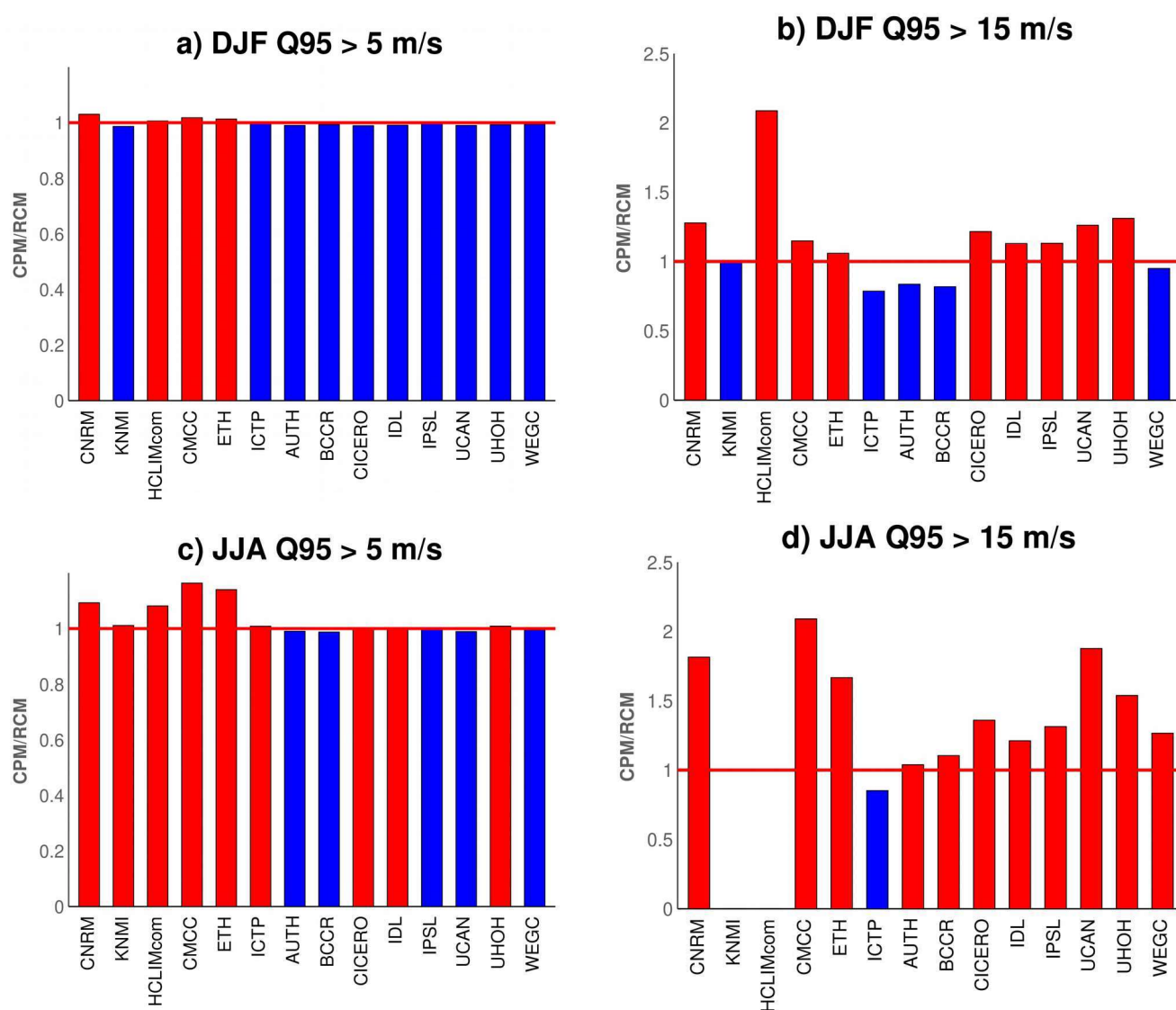
Figure 3. Ratio of frequency distribution of spatial Q95 (95 th percentile) of the wind speed for all available pairs of CPM-RCM simulations. First row (a, b) cold season (DJF), second row (c, d) warm season (JJA). (a, c) Q95 > 5 m/s, (b, d) Q95 > 15 m/s. Red bars indicate CPM v. RCM ratio larger than 1, while blue bars indicate ratio smaller than 1.
