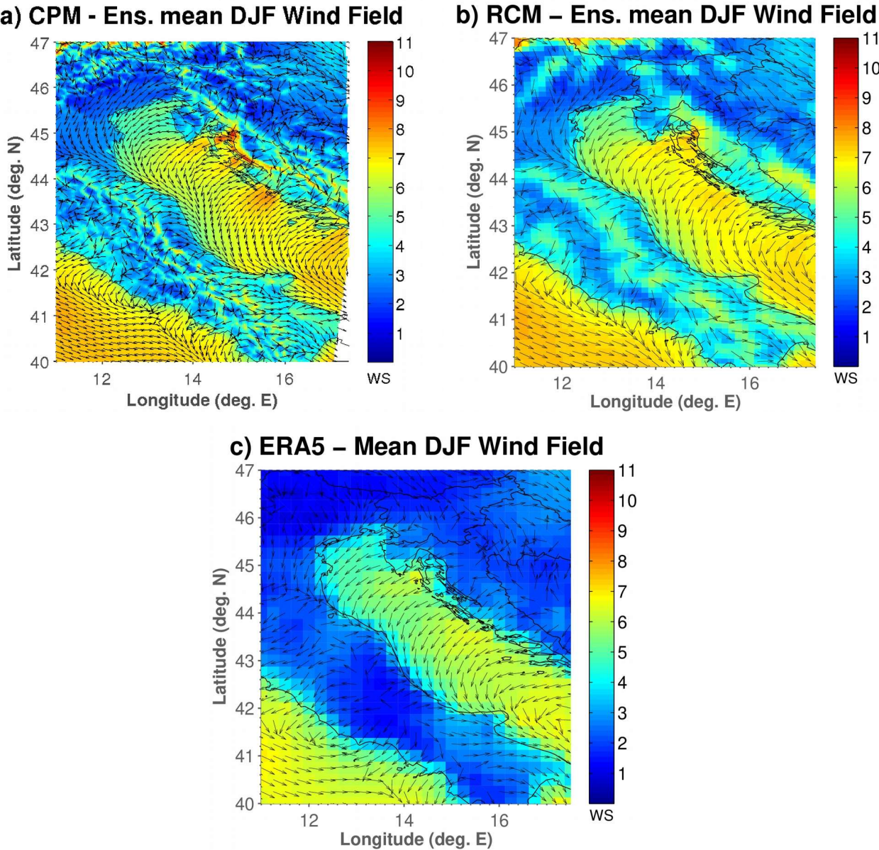
Figure 2. Cold season (DJF) spatial mean of wind speed (colors) and normalized wind direction (black arrows) for a) CPM ensemble, b) RCM ensemble, c) ERA5. For the CPM ensemble every 6th, while for the RCM ensemble every 2nd vector is shown.
