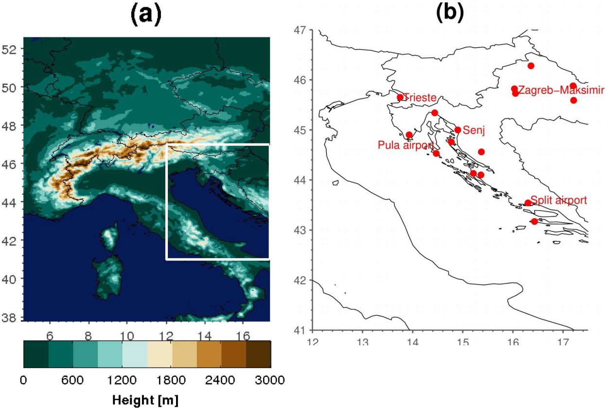
Figure 1. a) ALP-3 domain and the Adriatic domain (white box) used in this study. Colors correspond to topographic elevation in meters obtained from ICTP-RegCM4.7 CPM simulation. b) Adriatic domain with stations analyzed in this study in red dots. Names are associated with the stations mentioned in text.
