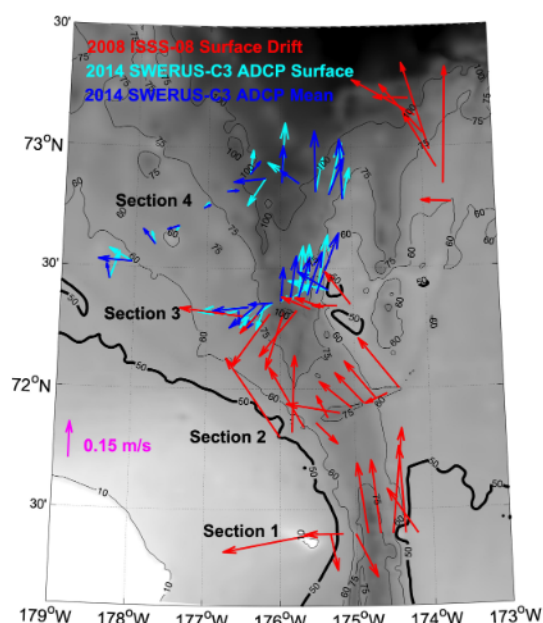
Figure 2. Circulation pattern in Herald Canyon and reference velocities for the geostrophic shear velocities. Shown are 2014 SWERUS-C3 vertical mean LADCP velocities (blue arrows), 2014 SWERUS-C3 surface LADCP velocities (cyan arrows), and 2008 ISSS-08 surface velocities from ship drift and navigation data (red arrows). Bathymetry (grey-scale shading and black contours) is from the International Bathymetric Chart of the Arctic Ocean (IB-CAO) version 4 (Jakobsson et al., 2020).
