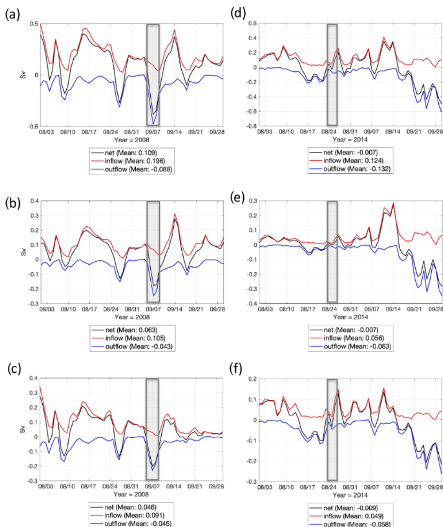
Figure 9. Daily modeled volume flux from the 9 km simulation across section 3 during August–September 2008 for all water masses (a), BSW only (b), and WW only (c), and during August–September 2014 for all water masses (d), BSW only (e), and WW only (f). The grey box shows the time period during which observations were collected. Inflow values are northward and outflow is southward. The mean values shown are for the 2-month time period (August–September).
