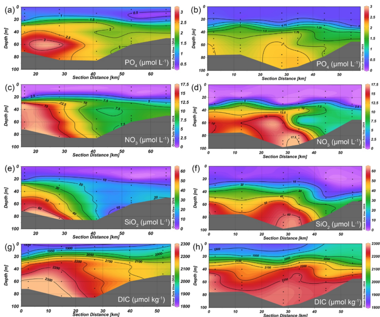
Figure 13. Observed nutrient and DIC sections at latitude about 72^{\circ}20' N (noted as 3 in Fig. 1b) in 2008 (a, c, e, g) and 2014 (b, d, f, h).
