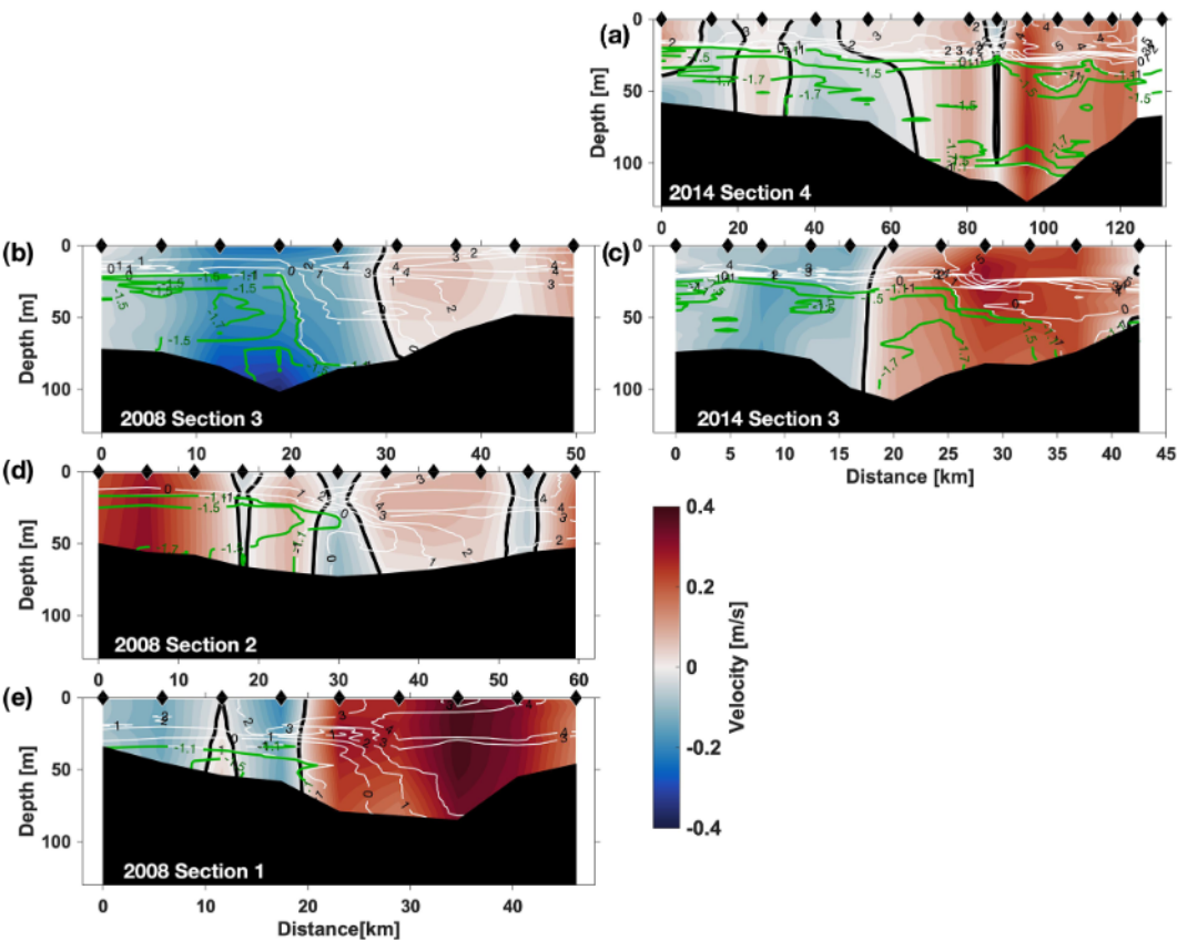
Figure 5. Cross-section velocities in 2008 for sections from north (b, d, e) and in 2014 (a, c). Shown in all panels is geostrophic shear referenced to the cross-section component of de-tided surface velocities from ship’s drift (2008) and LADCP (2014). The white contours show temperature from -1 to 8^{\circ}\text{C} at 1^{\circ}\text{C} intervals; the green ones show temperature from -1.3 to -1.7^{\circ}\text{C} at 0.2^{\circ}\text{C} to highlight the temperature structure within the WW. Please note that all sections cover different horizontal distances.
