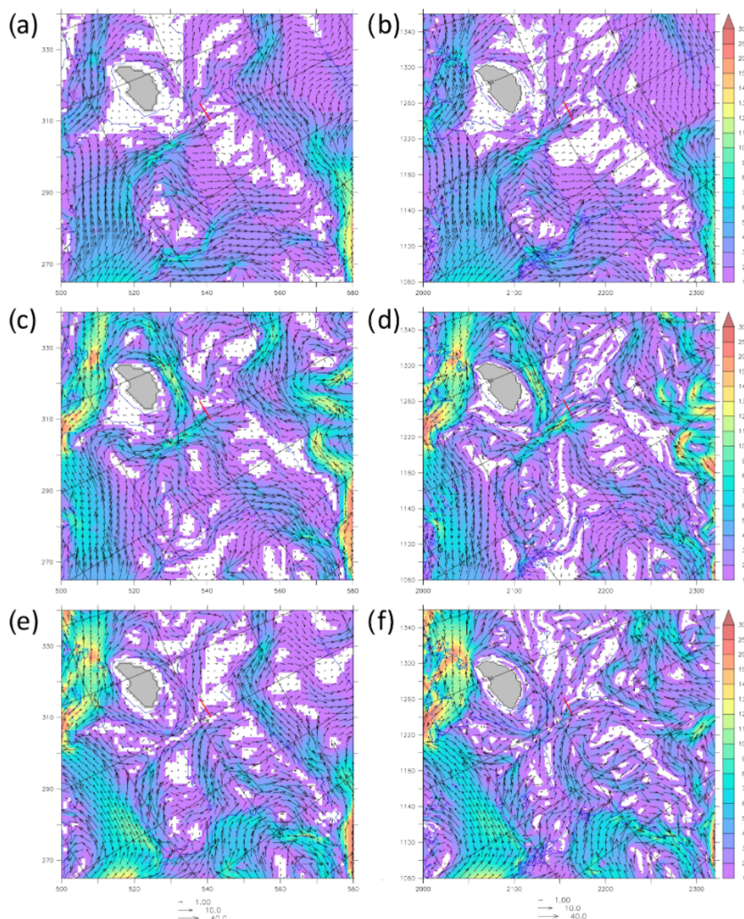
Figure 8. Upper 100 m averaged speed (shading) and velocity vectors ( \text{cm s}^{-1} ) from model output. The left column (a, c, e) is from the 9 km model results and the right column (b, d, f) is from the 2 km model results. The top row (a, b) is a 10-year mean from 2006–2015. The middle row (c, d) is a mean for September 2008. The bottom row (e, f) is a mean for August 2014. Every second vector for 9 km and every eighth vector for 2 km is shown. Blue lines indicate isobaths at 25, 50, 100, and 1000 m. The red line indicates the location of section 3 discussed elsewhere. The x and y axes are labelled with model grid cell numbers.
