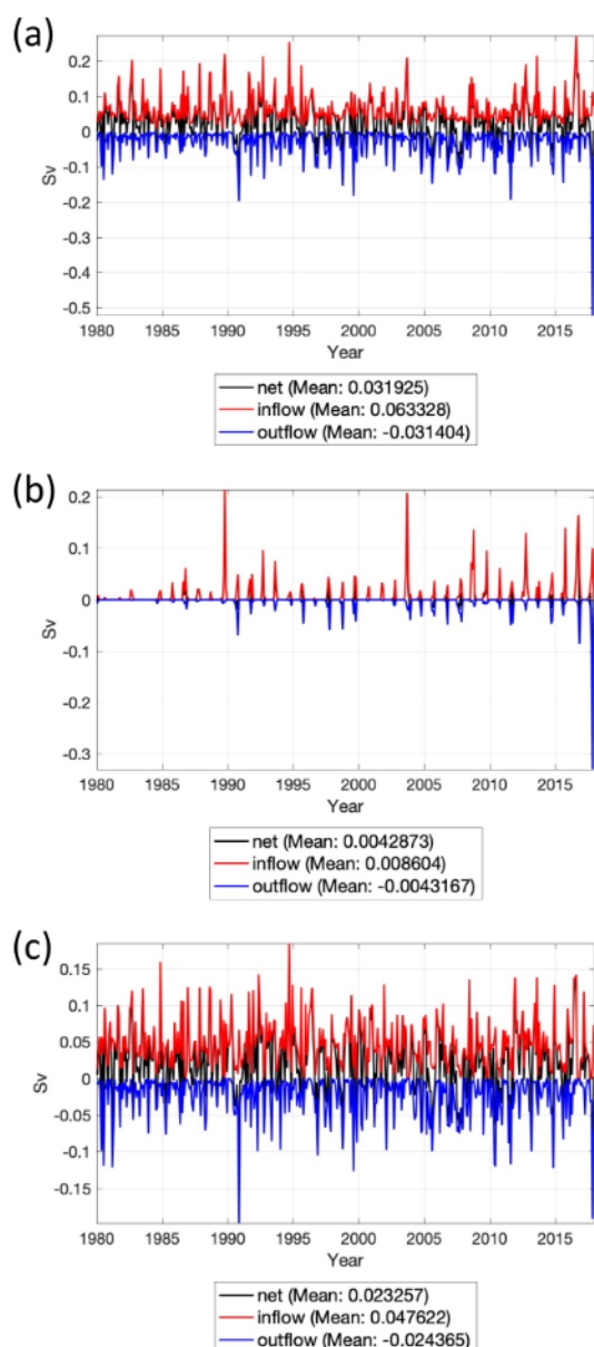
Figure 12. Monthly mean modelled volume flux ( S_v ) from the 9 km simulation across section 3 during 1980–2017 for all water masses (a), BSW only (b), and WW only (c). Inflow values are northward and outflow is southward.
