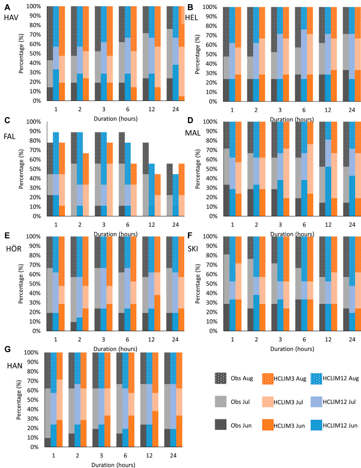
FIGURE 7 | Percentage of annual extremes \text{Perc}_{\max}^d in Jun, Jul and Aug for durations 1, 2, 3, 6, 12, and 24 h in stations HAV (A), HEL (B), FAL (C), MAL (D), HÖR (E), SKI (F) and HAN (G).
