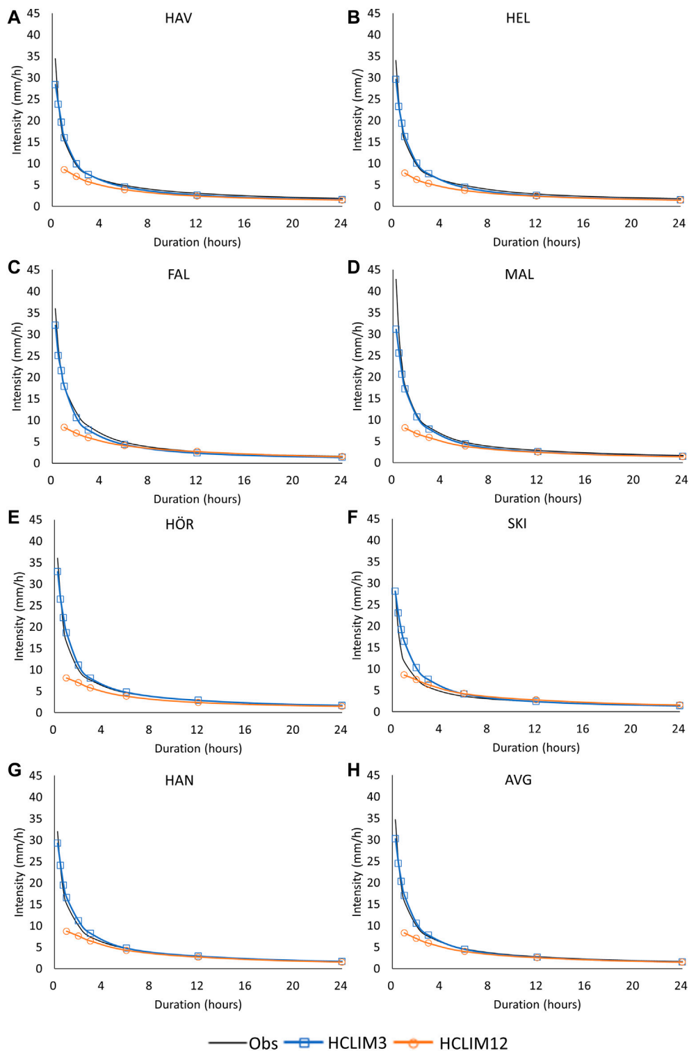
FIGURE 6 | Intensity-Duration curves of observed and simulated average annual maxima in stations HAV (A), HEL (B), FAL (C), MAL (D), HÖR (E), SKI (F) and HAN (G) as well as on average over all stations (H).
