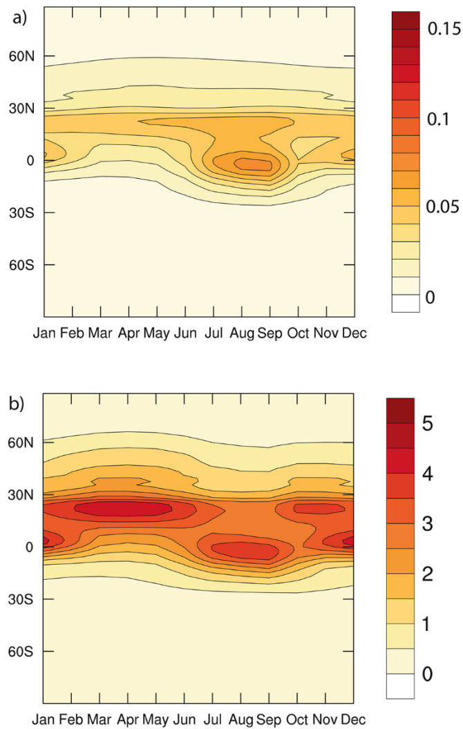
Fig. 7. MACv2-SP \tau_a patterns in 2020. Shown are the annual cycles of the anthropogenic aerosol optical depth ( \tau_a ) at 550 nm as (a) zonal means and (b) zonal means weighted by \tau_a for the two-year-blip scenario.
