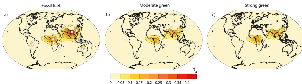
Fig. 3. MACv2-SP \tau_a in 2050. Shown is the annual mean in anthropogenic aerosol optical depth ( \tau_a ) at 550 nm for the (a) fossil-fuel based, (b) moderate green, and (c) strong green scenario. Grey symbols mark the centers of the aerosol plumes associated with industrial pollution (circles) and emissions from both industry and biomass burning (rectangles).
