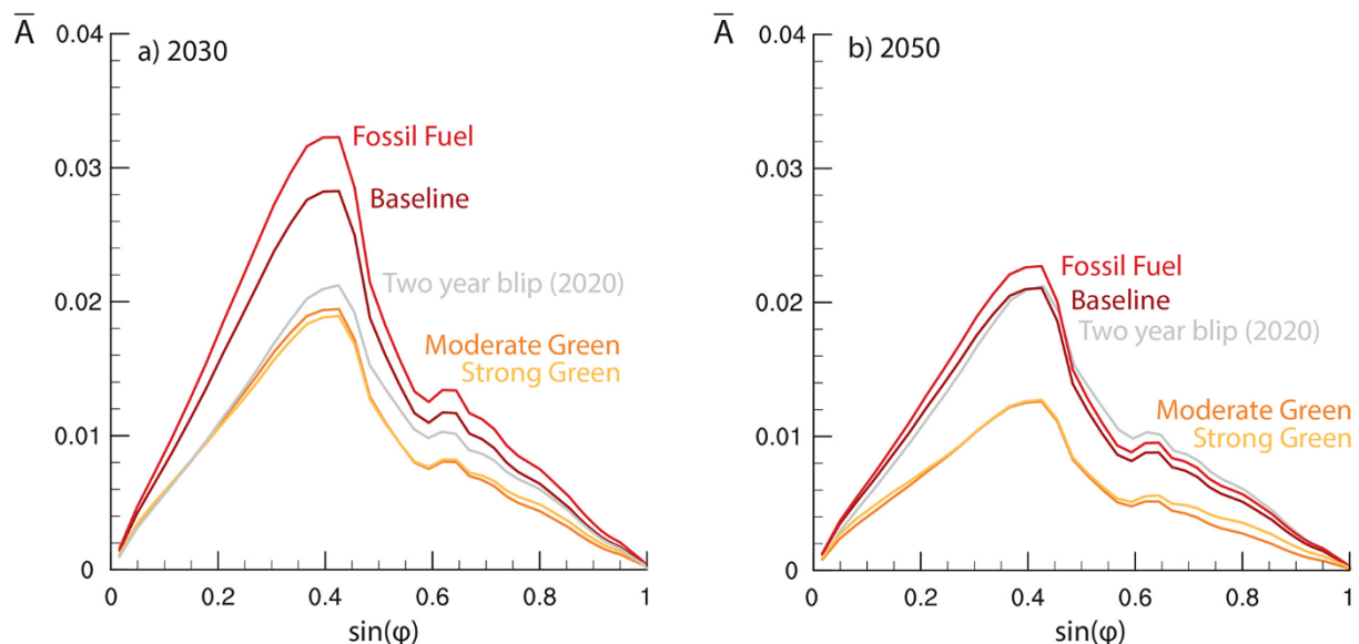
MACv2-SP \tau_a . Shown is the hemispheric asymmetry ( A ) as function of the sinus of the geographical latitude for (a) 2030 and (b) 2050. The two-year blip are identical for these years. We mark the values of the two-year blip scenario in 2020 as a reference.
