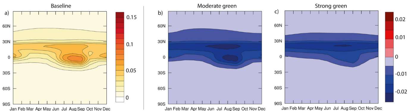
Fig. 8. 2050. Shown is the annual cycles of the anthropogenic aerosol optical depth ( \tau_a ) at 550 nm as (a) zonal mean for the baseline, and (b) moderate green scenario and (c) strong green scenario relative to baseline for 2050.
