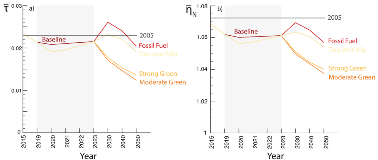
Fig. 5. MACv2-SP \tau_a in 2015–2050. Shown are the global annual means in (a) the anthropogenic aerosol optical depth ( \tau_a ) at 550 nm and (b) the scaling factor for inducing aerosol effects on clouds ( \eta_N ) for the scenarios. The pandemic period 2019–2023 is marked with grey shading. The baseline and two-year blip scenario except baseline overlap for 2015–2030. The 2005 value from the historical scaling is marked as horizontal line.
