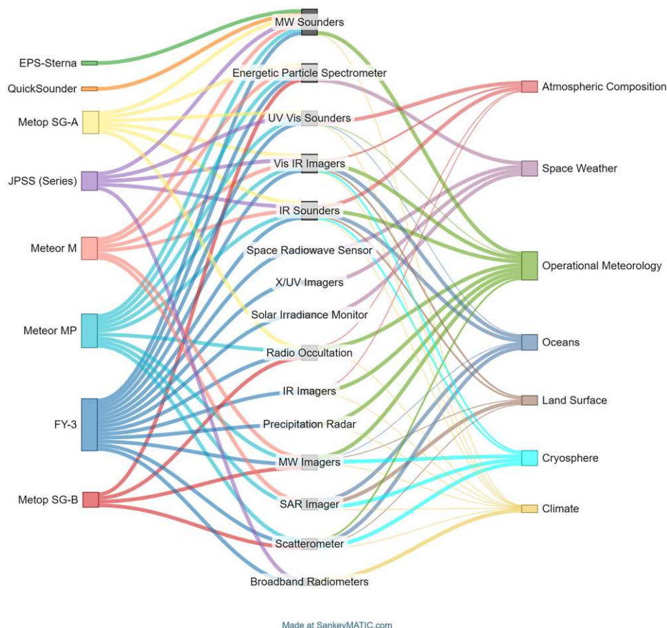
FIG. 4. Planned and new operational LEO missions covering the period 2020–50. Missions selected according to contributions to the WIGOS initiative from operational space agencies, determined by membership in the CGMS, as of 2020. (left) Names of missions. (center) A list of instrument classifications, taken from the WMO-OSCAR space-based capabilities. (right) Broad categories of applications across the different Earth systems. Connections between the right and center columns are determined by the payloads of the missions though they may represent more than one instrument. The connections between the center and left columns are determined by the authors' understanding of how important each instrument type's contribution is to the communities surrounding each application area. Each mission is connected by a unique colored line to each instrument it possesses and then to each application area by another unique colored line. Connections to climate are based on observational value to the creation of long-term climate records. Planned instrument information is collected from WMO-OSCAR and is correct up to March 2024. Note: Feng-Yun-3 (FY-3) includes FY-3E-I . JPSS includes NOAA-21 but no additional planned follow-up(s) from the NEON program.
