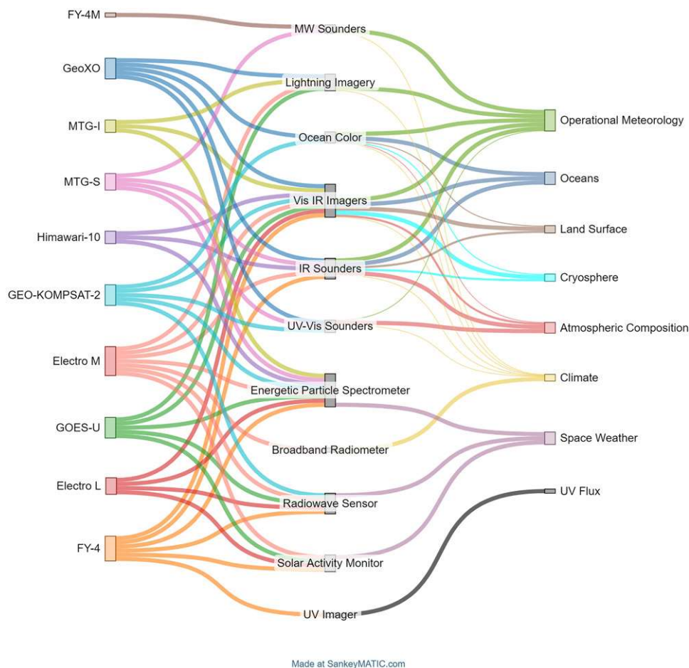
FIG. 3. Planned and new operational geostationary (GEO) missions covering the period 2020–50. Missions selected according to contributions to the WIGOS initiative from operational space agencies, determined by membership in the CGMS, as of 2020. (left) Names of missions. (center) A list of instrument classifications, taken from the WMO-OSCAR space-based capabilities. (right) Broad categories of applications across the different Earth systems. Connections between the right and center columns are determined by the payloads of the missions though they may represent more than one instrument. The connections between the center and left columns are determined by the authors' understanding of how important each instrument type's contribution is to the communities surrounding each application area. Each mission is connected by a unique colored line to each instrument it possesses and then to each application area by another unique colored line. Connections to climate are based on observational value to the creation of long-term climate records. Planned instrument information is collected from WMO-OSCAR and is correct up to March 2024. Note: Feng-Yun-4 (FY-4) includes FY-4B–E. GeoXO includes the East/West and Central missions. GEO-KOMPSAT-2 includes both the GEO-KOMPSAT-2A and GEO-KOMPSAT-2B missions.
