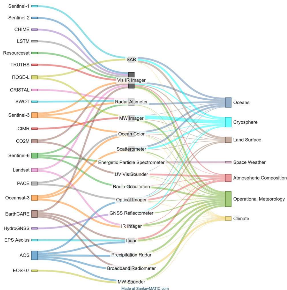
FIG. 5. Planned and new topical missions covering the period 2020–50. Missions selected according to contributions to the WIGOS initiative from operational space agencies, determined by membership in the CGMS, as of 2020. (left) Names of missions. (center) A list of instrument classifications, taken from the WMO-OSCAR space-based capabilities. (right) Broad categories of applications across the different Earth systems. Connections between the right and center columns are determined by the payloads of the missions though they may represent more than one instrument. The connections between the center and left columns are determined by the authors' understanding of how important each instrument type's contribution is to the communities surrounding each application area. Each mission is connected by a unique colored line to each instrument it possesses and then to each application area by another unique colored line. Connections to climate are based on observational value to the creation of long-term climate records. Planned instrument information is collected from WMO-OSCAR and is correct up to March 2024.
