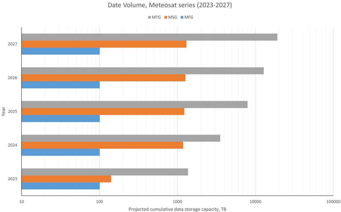
FIG. 1. Cumulative data storage (TB) volume, budgeted for each of the EUMETSAT geostationary programs (Meteosat) over the period 2023–27. MFG: Meteosat First Generation. Note: The scale is exponential.
