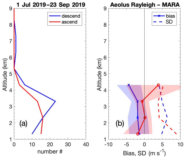
Figure 4. Height profiles in 1 km bins of (a) the number of comparison points available and (b) mean value (bias) and standard deviation of the differences between Aeolus Rayleigh HLOS winds and MARA-derived HLOS winds for the Antarctic winter period 1 July–23 September 2019. Red lines and shading are for ascending tracks and blue is for descending ones. Solid lines in (b) show the bias, with the shaded areas corresponding to the 90 % confidence interval. Dashed lines in (b) show the standard deviation.
