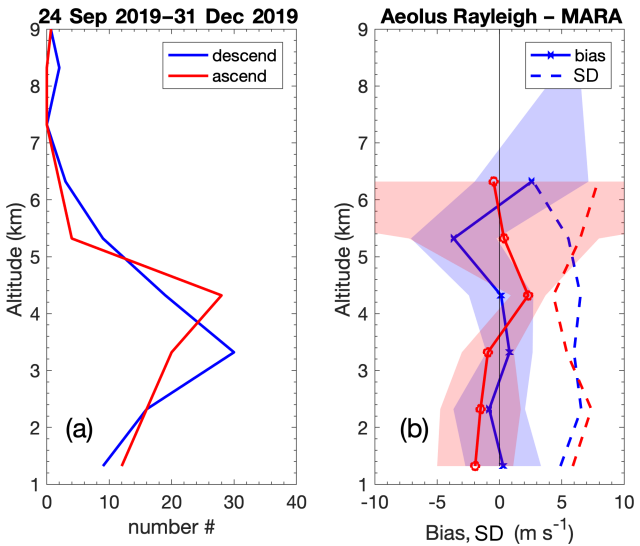
Figure 5. The same as Fig. 4. but for Aeolus Rayleigh HLOS winds and MARA-derived HLOS winds for the Antarctic summer period 24 September–31 December 2019.
