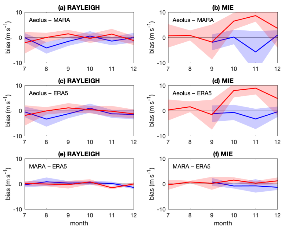
Figure 9. Month-by-month mean values of biases in HLOS winds (solid lines) and 90 % confidence limits (shaded areas) at MARA. Red is for ascending tracks and blue is for descending ones. (a) Aeolus Rayleigh minus MARA, (b) Aeolus Mie minus MARA, (c) Aeolus Rayleigh minus ERA5, (d) Aeolus Mie minus ERA5, (e) MARA minus ERA5 at available Aeolus Rayleigh comparison times/heights and (f) MARA minus ERA5 at available Aeolus Mie comparison times/heights.
