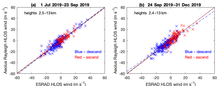
Figure 10. Scatter plots of Aeolus Rayleigh HLOS winds against HLOS winds according to ESRAD radar data. Red crosses indicate measurements made on ascending tracks and blue crosses are for descending tracks. Dashed red and blue lines show fitted regression lines. Black dashed line indicates equality. Heights indicated are the lowest and highest where valid winds are available for comparison. (a) The Arctic summer period 1 July–23 September 2019; (b) winter 24 September–31 December 2019.
