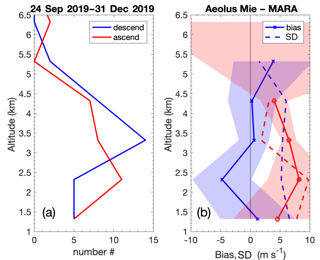
Figure 8. The same as Fig. 5 but for Aeolus Mie HLOS winds against MARA (summer).
