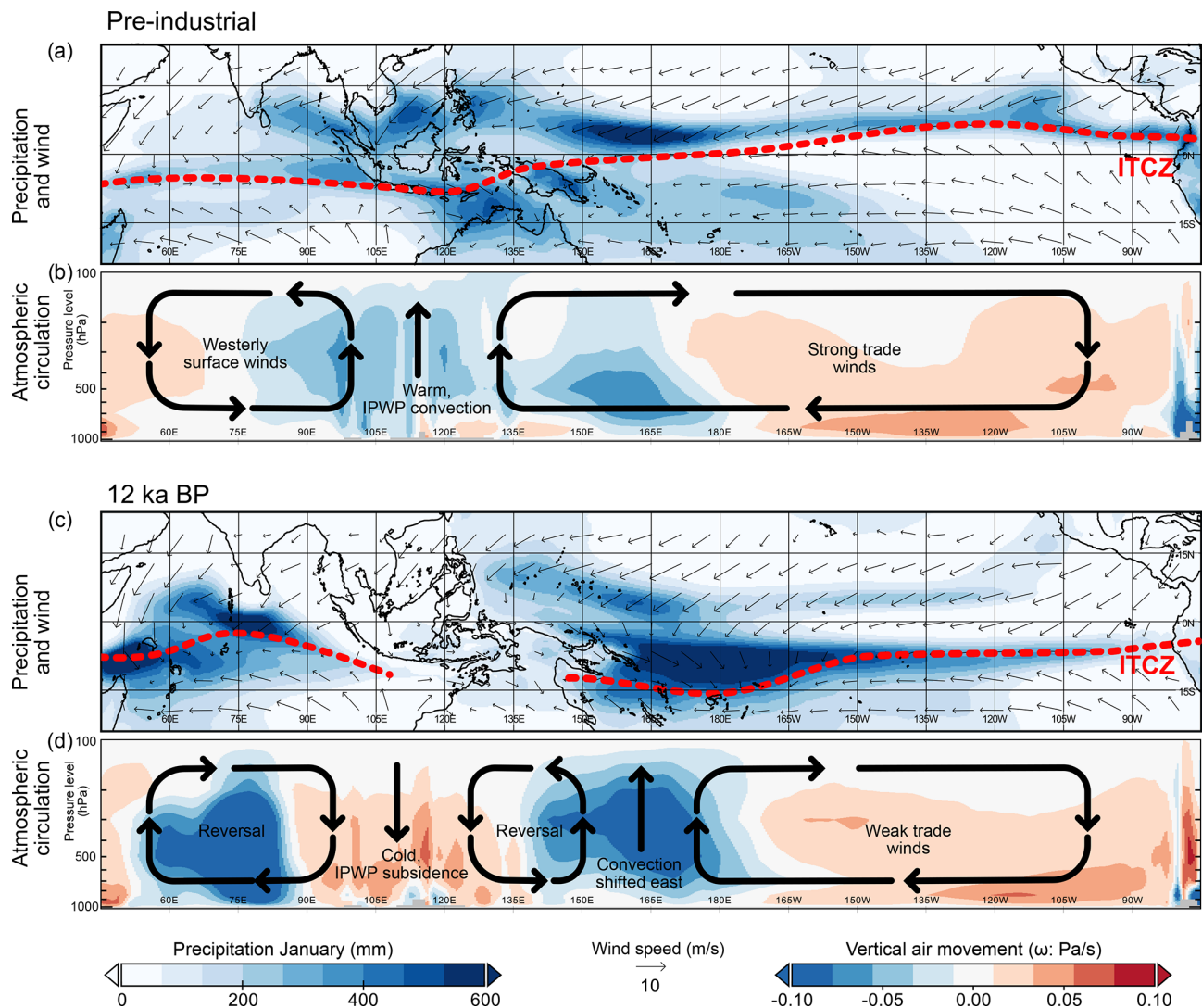
Figure 5. Simplified mechanistic explanation for January precipitation patterns during the preindustrial ( a , b ) and 12 ka BP ( c , d ) in terms of horizontal and vertical wind patterns. ( a ) and ( c ) show mean total precipitation (mm per month) and surface wind vectors ( \text{m s}^{-1} ) for January; ( b , d ) Omega parameter ( \omega: \text{Pa s}^{-1} ) representing vertical air movement ( \omega < 0 , rising in blue; \omega > 0 sinking in red) along the Equator over the Indo-Pacific region. The approximate January location of the ITCZ and atmospheric Walker Circulation patterns are indicated as red lines ( a , c ) and black arrows ( b , d ), respectively. Note that the atmospheric circulation cells are inverted over the IPWP region at 12 ka BP where subsiding air masses, a breakdown of deep convection and divergent winds from land to sea cause seasonal aridity over tropical land areas. For details on the weakening and/or reversal of the zonal winds, see Fig. S7.
