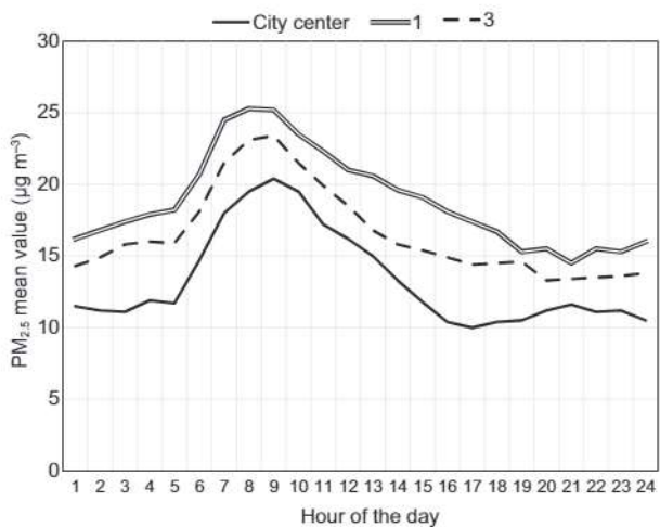
Fig. 7. Daily variation (mean values for different hours of the day) of monitored PM_{2.5} concentrations in the Vijes urban background for all hourly data for which also meteorological data were registered (to show the same data as in Fig. 6).
