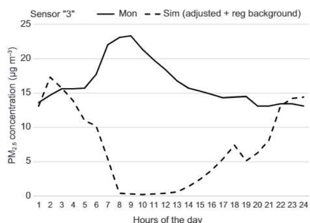
Fig. 9. Daily variation (mean values for different hours of the day) of monitored and simulated PM 2.5 concentrations summed from the industrial impact scaled by a factor of 60% plus a rural background value of 1 \mu\text{g m}^{-3} for all hours with a westerly wind component. Units: \mu\text{g m}^{-3} .
