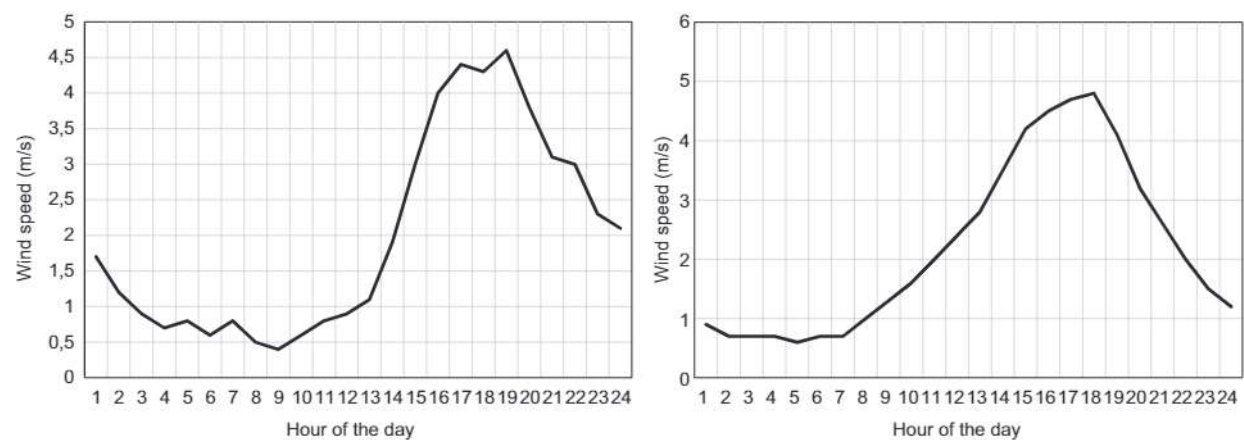
Fig. 4. Daily variation (mean values for each hour of the day on the x -axis) of wind speed in Vijes during the two monitoring campaigns. Left panel: January 28 to April 28, 2017 (1519 hourly data). Right panel: May 16 to October 25 (2044 hourly data).
