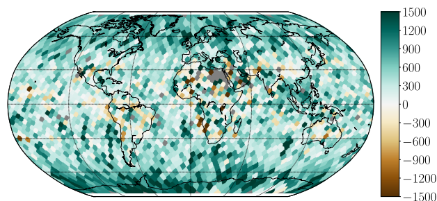
Figure 8. Mean absolute error difference in meters between MODIS-C6 and NN-AVHRR compared to CALIOP. Results are calculated for bins evenly spread out 250 km apart. Bins with fewer than 10 cloudy pixels are excluded (plotted in dark grey). Dark green means NN-AVHRR is 1.5 km better than MODIS-C6, dark brown means MODIS-C6 is 1.5 km better than NN-AVHRR. The final validation and testing under development data (see Table 1) are included to get enough pixels.
