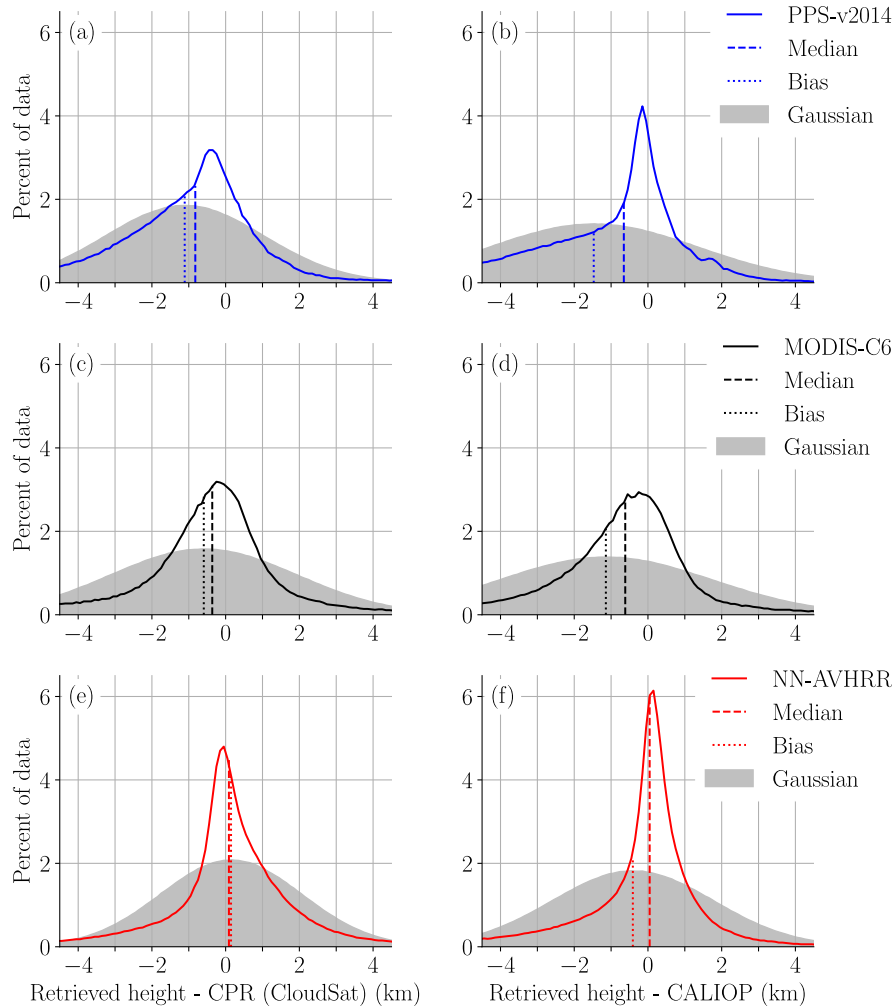
Figure 5. Error distribution compared to CPR (CloudSat) (a, c, e) and CALIOP (b, d, f) with biases and medians marked. The percent of data is calculated in 0.1 km bins. The final validation dataset (see Table 1) where all algorithms had a height reported is used. Note that the values on the y axis are dependent on the bin size. The peak at 6 % for NN-AVHRR in (f), means that 6 % of the retrieved heights are between the CALIOP height and the CALIOP height + 0.1 km. The Gaussian distribution with the same bias and standard deviation is shown in grey.
