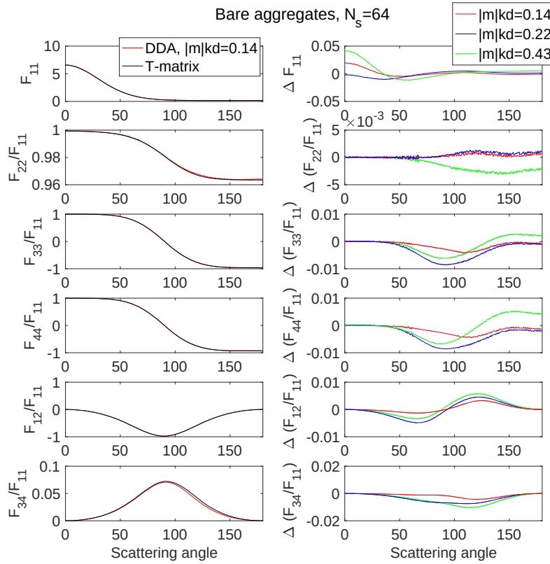
Fig. 3. Left column: Elements of the Stokes scattering matrix of bare BC aggregates composed of 64 monomers, computed with the superposition T-matrix method and analytic orientation averaging (black, reference case), and with the discrete dipole approximation (red), using a dipole spacing d with |m|kd=0.14 and 864 discrete orientation angles. Right: Differences between the DDA and the reference T-matrix results for |m|kd=0.14 (red), 0.22 (blue), and 0.43 (green).
