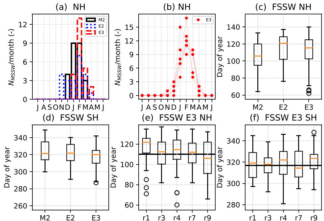
Figure 8. Number of major SSW (MSSW) as a function of the calendar month in the northern hemisphere (NH) for (a) for MERRA-2 (M2), EC-Earth2 (E2) and EC-Earth3 (E3), and (b) number of events in the EC-Earth3 five-member ensemble (note that dots are overlapping for some months). Boxplots of the final sudden stratospheric warming (FSSW) date in MERRA-2, EC-Earth2 and EC-Earth3 in the (c) NH and (d) southern hemisphere (SH). Outliers are indicated with circles. Boxplots for FSSW dates for all EC-Earth3 AMIP realizations in (e) the NH and (f) the SH, with dates for r10i1p1f1 shown with the horizontal line. Note that the EC-Earth2 record is \sim 10 years shorter than other data sets.
