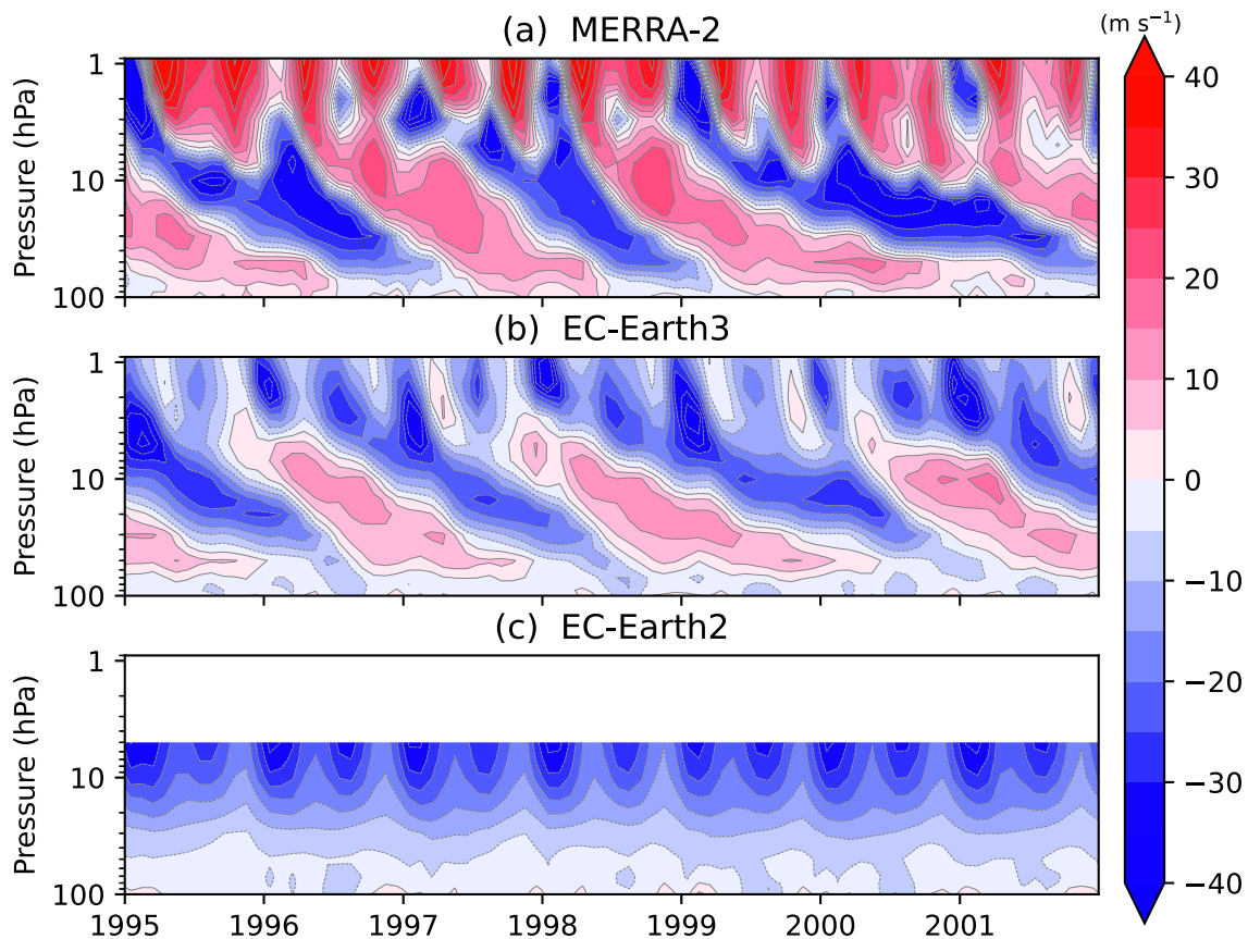
Figure 4. Zonal mean zonal wind in the equatorial stratosphere as a function of time and pressure for (a) MERRA-2, (b) EC-Earth3 and (c) EC-Earth2.
