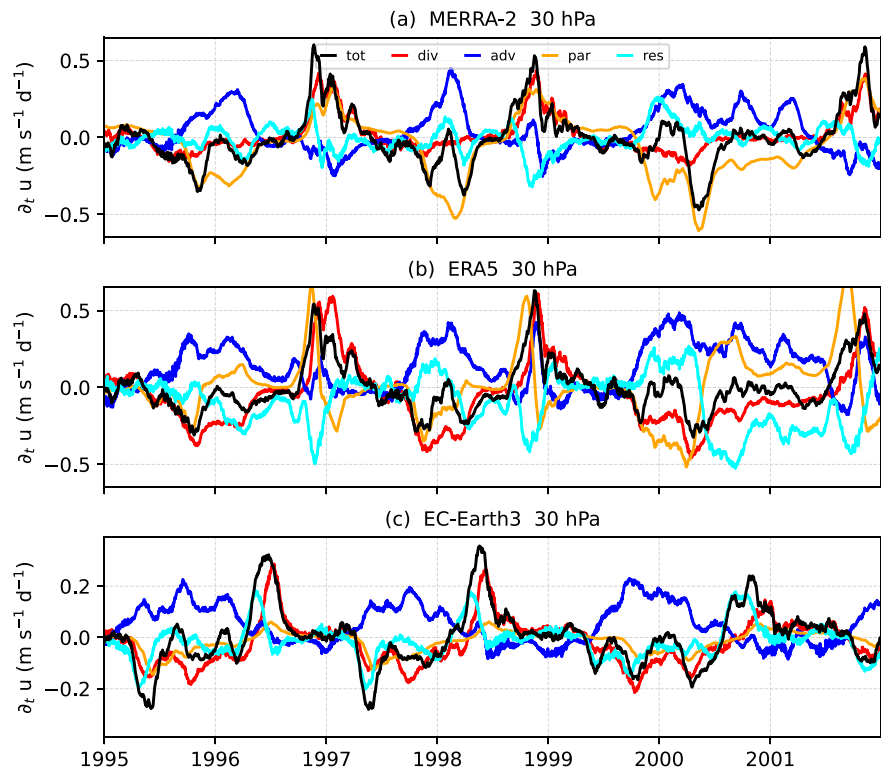
Figure 7. As in Figure 6, but for the 30 hPa pressure level. Note the different y-axis extent.
