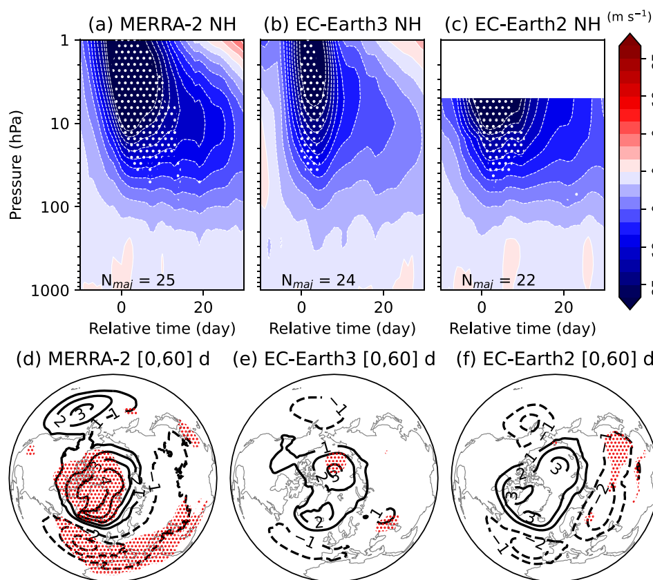
Figure 9. Time-pressure composites of the zonal mean zonal wind anomalies during northern hemisphere (NH) MSSWs in (a) MERRA-2, (b) EC-Earth3 and (c) EC-Earth2. The number of events for each data set is shown in the bottom left of each panel. Plots (d–f) report the corresponding NH sea level pressure (units hPa) composites between days 0–60 after MSSW central dates. Day zero marks the central date of the MSSW event, that is, the date of zonal wind reversal. In all plots, hatchings indicate significant differences at the 5% level based on bootstrapping of random winter dates.
