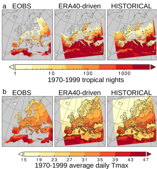
Fig. 5 a Number of tropical nights defined as days where the minimum temperature does not fall below 20 °C. b Average yearly maximum 2 m air temperature [°C]. Note that the E-OBS data set lacks data over open water
