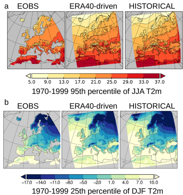
Fig. 6 a 95th percentile of summer 2 m air temperature calculated from the E-OBS data set, the coupled ERA40 hindcast run, and the climate scenario ensemble. b Same as (a) but displaying the 25th percentile of winter 2 m air temperature
