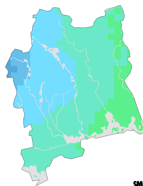
Observerat 1991-2013
