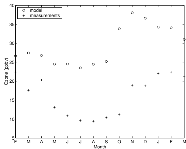
Fig. 2. Monthly means of ozone averaged over 36 non-remote stations from February 2001 to March 2002.
