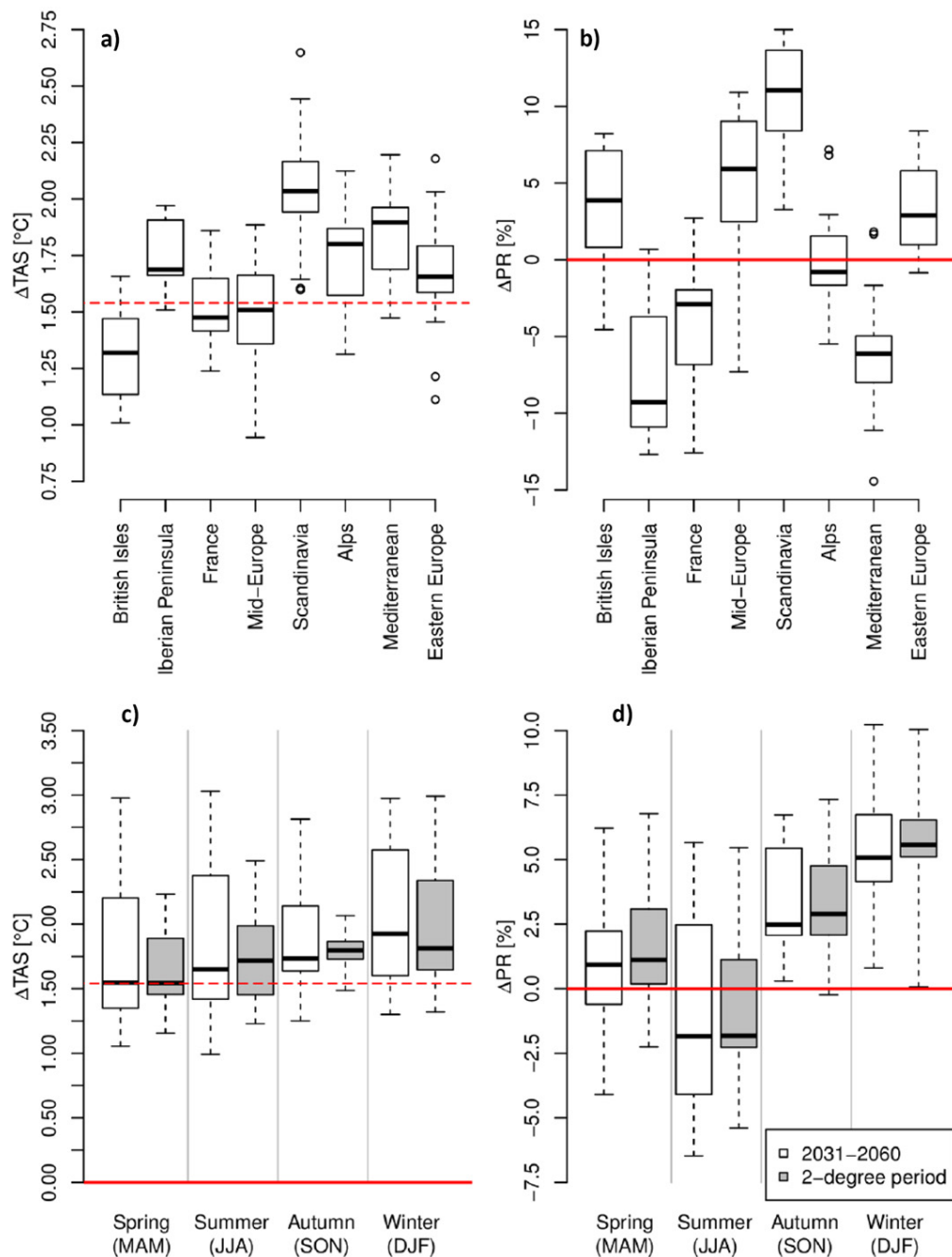
Figure 2. (a) Yearly averaged change—relative to the reference period 1971–2000—in yearly mean temperature in the different European regions for periods corresponding to +2 ^{\circ}\text{C} of global average change. The global temperature change (1.54 ^{\circ}\text{C} ) between 1971–2000 and the 2 ^{\circ}\text{C} period is marked as a dotted line. (b) Same as (a) for precipitation in % of change. The solid red line indicates no change for precipitation and the red dotted line a change of 1.54 ^{\circ}\text{C} for temperature, corresponding to a global warming of 2 ^{\circ}\text{C} relative to pre-industrial. (c) Spatial average over land of changes in temperature and (d) precipitation, together with the range of changes for the GCM–RCM ensemble (median, 25–75% range and min and max values). The open bars refer to fixed time future period (2031–2060), the gray bars to the temperature controlled (+2 ^{\circ}\text{C} ) period.
