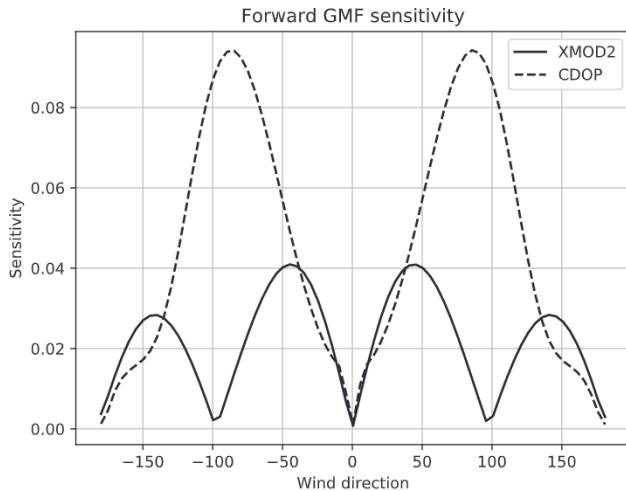
Fig. 20. GMF sensitivity ( \partial F / \partial \rho_w ) as a function of WD. 0° upwind, \pm 180^\circ downwind, \pm 90^\circ crosswind.
