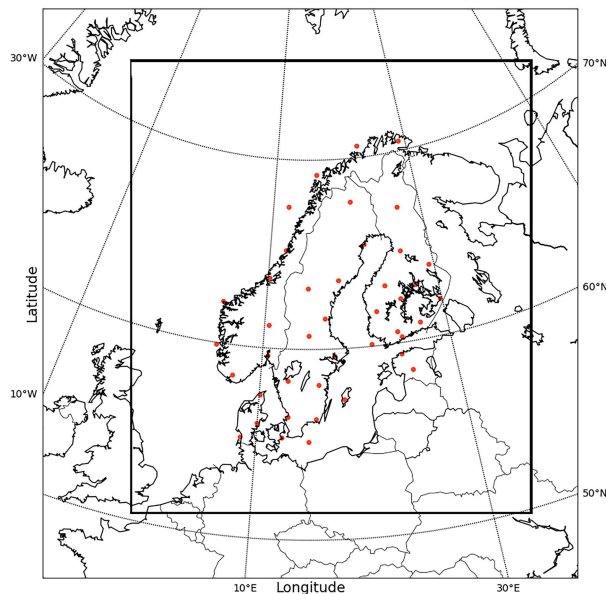
FIG. 1. The MetCoOp operational model domain and the domain used in the experiments in this study. The locations of the included radar stations are indicated by the red dots.
