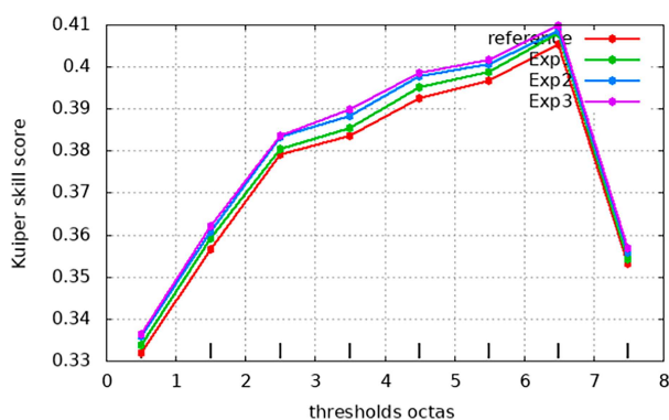
FIG. 14. KSS for cloud cover for the reference experiment (red), Exp1 (green), Exp2 (blue), and Exp3 (purple) against the number of octas of the sky covered by clouds.
