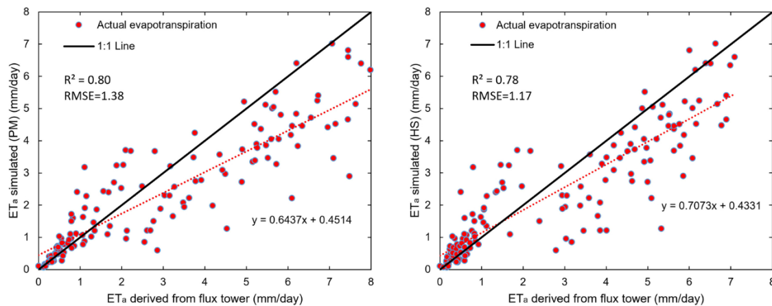
Fig. 5. Relationship between measured and calculated actual evapotranspiration using Penman–Monteith (PM) and Hargreaves and Samani (HS) equations for 2018 during the crop-growing season. The measured data was from Lanna ICOS station in 2018.
