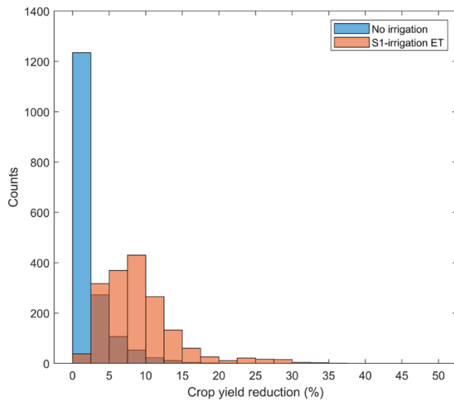
Fig. 14. Crop yield reduction due to temperature stress for no irrigation and for scenario S1-irrigation ET in 2018.
