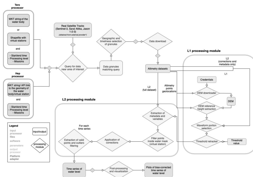
Figure 3. Water level processor teroWAT diagram block.
