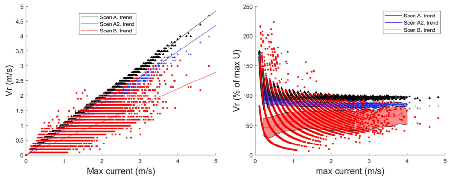
Fig. 9. Rated tidal-stream turbine speed using standardised power density curve and three optimal solutions: Scenario A (maximum yield density shown in black), Scenario A2 (high yield density shown in blue) and Scenario B (firm power shown in red).
