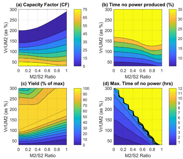
Fig. 6. Performance of multiple tidal-stream power curves, represented here as rated speed ( V_r ) relative to the resource (amplitude of M2 harmonic: UM_2 ), for a given site where the tidal currents are controlled solely by the spring-neap cycle and the ratio of M2 and S2 amplitude ( M_2/S_2 of 0 has only an M2 tide, whilst equal M2 and S2 current amplitudes has a ratio of 1). Turbine performance is described using Capacity Factor (a), percentage of time no power produced (b), (c) mean yield density (relative to maximum possible) and (d) the longest period of zero power in a 15 day time-series.
