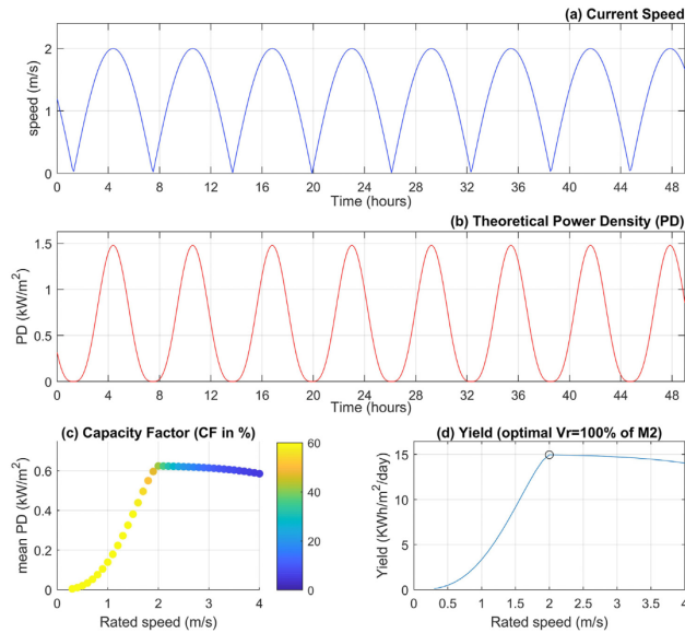
Fig. 4. Single harmonic tidal current (M2 amplitude 2 m/s) over a 2 day period (panel a), and the theoretical power density (PD) of this current (panel b), compared to the mean power density and Capacity Factor (panel c) for multiple tidal-stream turbine power curves, where rated power is capped at rated speed ( V_r ), and cut-in speed is 30% of V_r , which allows mean daily yield density to be calculated (panel d).
