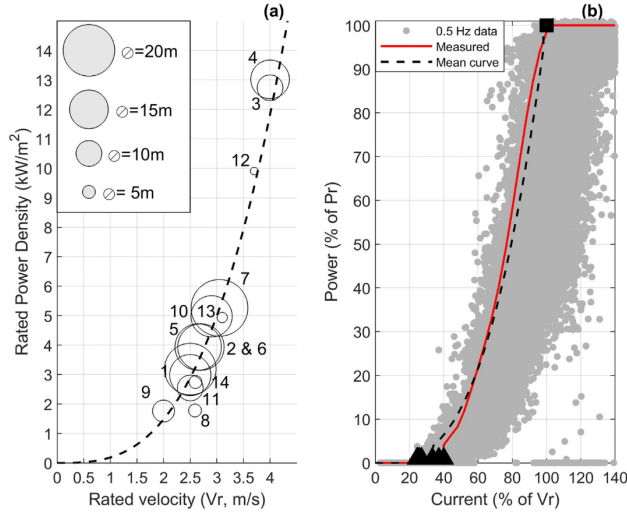
Fig. 2. Tidal-stream turbine characteristics from 14 commercially developed devices (panel a), normalised (relative to rated power and speed) and compared to observed variability (grey dots and averaged power curve in red) from a grid-connected device in Lewis et al. [6].
