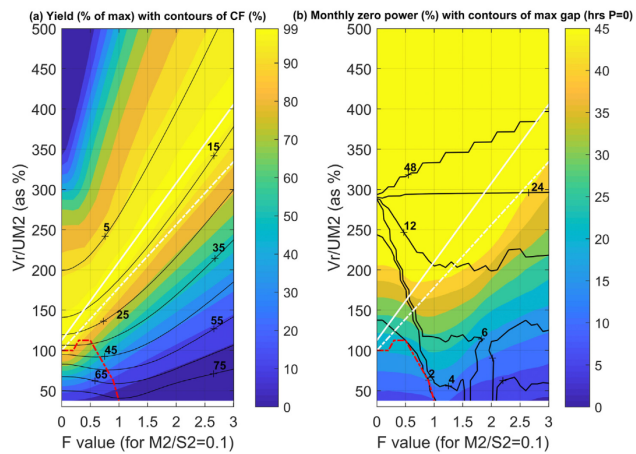
Fig. 7. Tide currents harmonic characteristic tidal form (F value), rated turbine speed (relative to M2 current amplitude UM_2 ) and subsequent yield and Capacity Factor (CF) shown in panel a, with mean monthly percentage of zero power and maximum period of no power (max gap) in panel b. Lines of optimal power curve shown in solid white for selection of maximum yield (Scenario A), high yield (scenario A2) as dashed white line and firm power (power gap < 2 h with highest CF: scenario B) as red dashed line.
