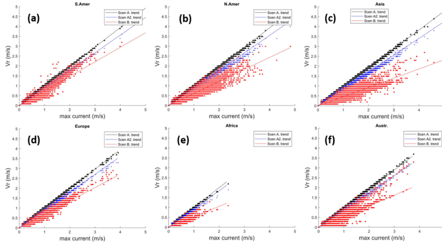
Fig. A3. The optimal rated tidal-stream turbine speed, for three scenarios (a to c for max, high and firm yield respectively), based on FES2014 global data and grouped into the 6 continents: South America (a), North America (b), Asia (c), Europe (d), Africa (e), Australasia (f).
