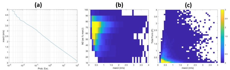
Fig. 8. Global variability of tidal dynamics, described as maximum flow (maxU) percentage exceedance (a) for sites “coastally” (<25 km offshore) resolved in the FES2014 data, (b) coloured percentage occurrence of M2 amplitude contribution to the maximum flow (as percentage of M2 current amplitude compared to maximum current speed), and (c) coloured percentage occurrence of the tidal form (F value) that describes the diurnal (F > 3) to semi-diurnal (F < 0.25) nature of the tide.
