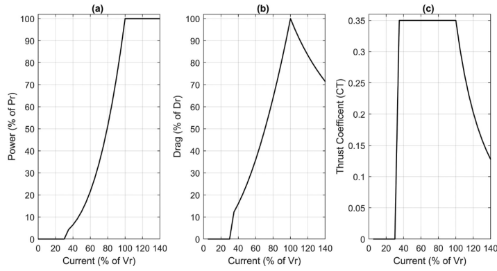
Fig. 3. A standardised power curve, based on 14 horizontal axis tidal-stream turbines, with the associated Drag (as percentage of maximum drag, Dr) and Thrust Coefficient (CT) normalised curves.
