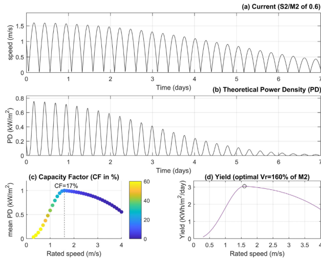
Fig. 5. Spring-Neap tidal current (M2 amplitude 1 m/s, S2 amplitude 0.6 m/s) over a 7 day period (panel a), with the theoretical power density (PD) of this current (panel b). Multiple tidal-stream turbine power curves, where rated power is capped at rated speed ( V_r ), and cut-in speed is 30% of V_r , are applied to resolve an optimal design using mean power density and Capacity Factor (panel c) and mean daily yield density (panel d).
