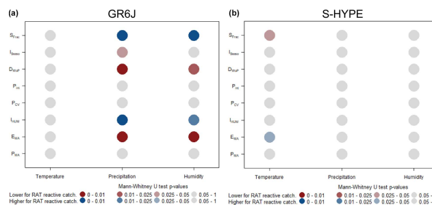
Figure 9. Results of the Mann–Whitney U test to evaluate the differences in climatic signatures in Sweden. The left plot represents differences between Swedish catchments in which GR6J reacts and catchments in which it does not, and the right plot represents differences between catchments in which S-HYPE reacts to the RAT and catchments in which it does not. The number of catchments in each subset can be found in Fig. 8. Blue (red) squares mean that the signature is significantly higher (lower) for reactive catchments. P_{MA} : mean annual precipitation, E_{MA} : mean annual evaporation, I_{HUM} : humidity index, P_{CV} : precipitation variability, P_{int} : precipitation intensity index, D_{WOP} : ratio of days without precipitation, I_{Seaso} : seasonality index and S_{Frac} : snow fraction.
