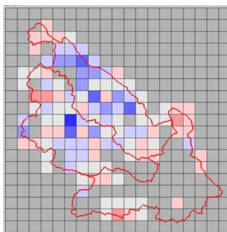
SCA: Simulated - observed, 1998/1999
