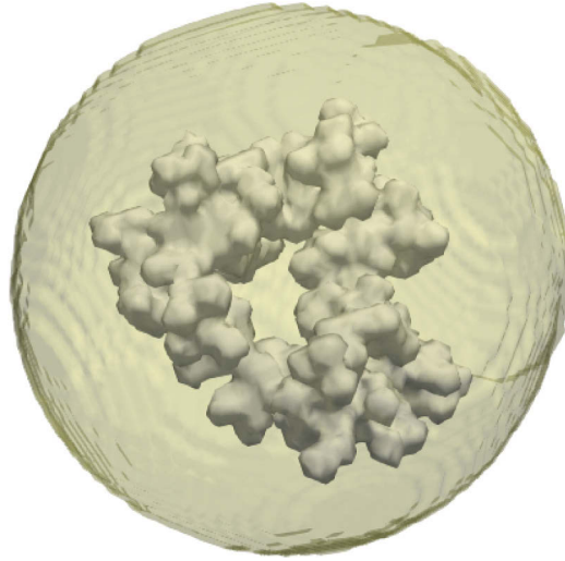
Fig. 1. Example of a coated soot aggregate consisting of N=286 overlapping monomers as used in the calculations. The aggregate is shown in grey and the coating shell in yellow.
