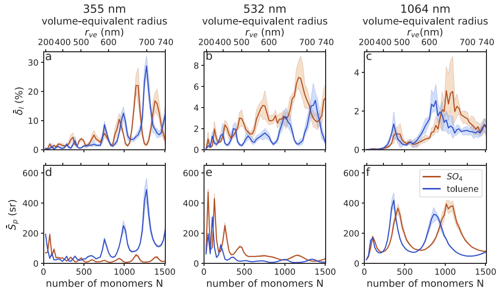
Fig. 2. Linear depolarisation ratio (a–c) and extinction-to-backscatter ratio (d–f) for sulphate coating (red/light red) and toluene-based coating (blue/light blue) for 355 nm (a, d), 532 nm (b, e) and 1064 nm (c, f). The arithmetic mean over five different stochastic realisations of the aggregates is shown in red and blue, respectively. The shading indicate the range due to different stochastic realisations of the aggregate structure.
