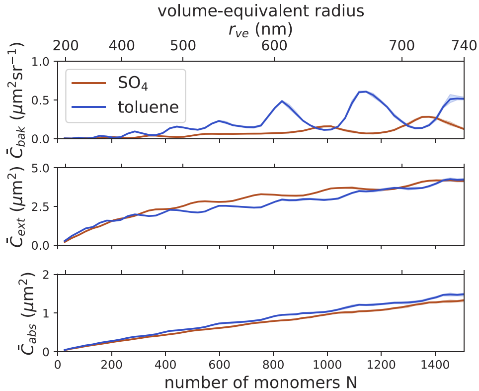
Fig. 3. Backscattering ( C_{bak} , top), extinction ( C_{ext} , centre) and absorption cross section ( C_{abs} , bottom) of the coated aggregates for sulphate coating (red) and toluene-based coating (blue) in \mu\text{m}^2 (for C_{ext} and C_{abs} ) and \mu\text{m}^2\text{sr}^{-1} (for C_{bak} ) at \lambda = 532 nm. Solid lines indicate the mean over the five different stochastic realisations and the shading the maximum uncertainty due to the different realisations of the stochastic geometries (The differences for the extinction and absorption cross section are too small to be distinguished from the mean).
